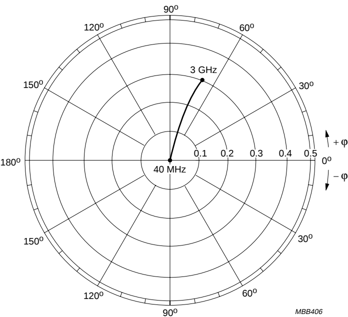
Fig.16 Common emitter reverse transmission coefficient ( S_{12} ).
