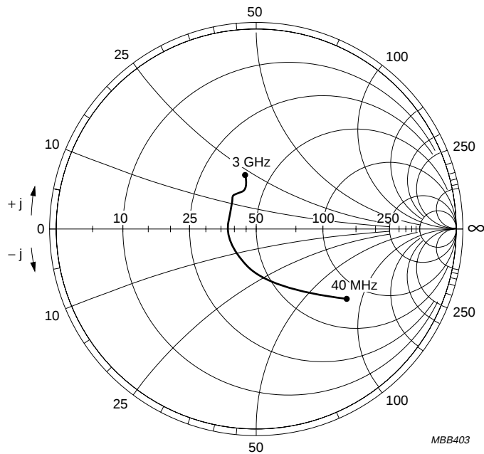
Fig.14 Common emitter input reflection coefficient ( S_{11} ).
