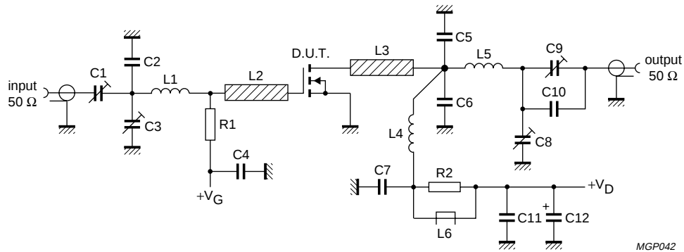
Fig.11 Test circuit for class-A operation.
