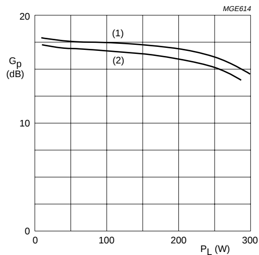
Class-AB operation; V_{DS} = 50 V; I_{DQ} = 2 \times 0.5 A; f = 225 MHz; Z_L = 0.74 + j2 \Omega (per section); R_{GS} = 2.8 \Omega (per section). (1) T_h = 25 °C. (2) T_h = 70 °C.
