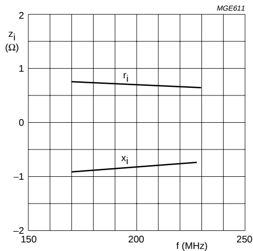
Class-AB operation; V_{DS} = 50\text{ V} ; I_{DQ} = 2 \times 0.5\text{ A} ; R_{GS} = 2.8\text{ }\Omega (per section); P_L = 250\text{ W} . Fig.23 Input impedance as a function of frequency (series components), typical values per section.
