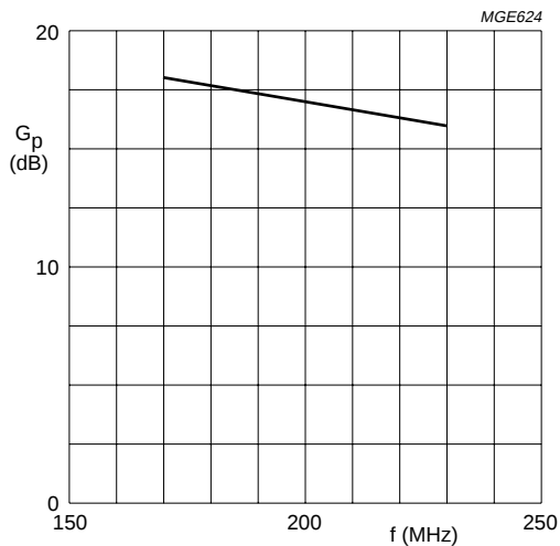
Class-AB operation; V_{DS} = 50\text{ V} ; I_{DQ} = 2 \times 0.5\text{ A} ; R_{GS} = 2.8\text{ }\Omega (per section); P_L = 250\text{ W} . Fig.26 Power gain as a function of frequency, typical values per section.
