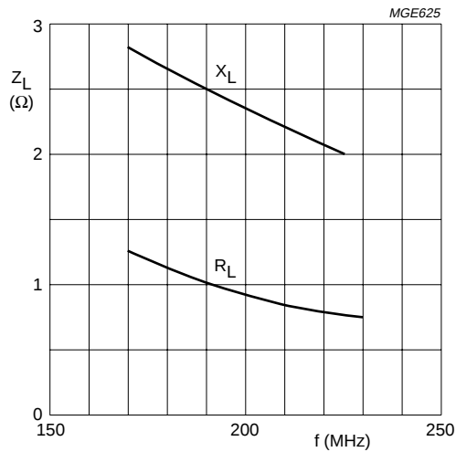
Class-AB operation; V_{DS} = 50\text{ V} ; I_{DQ} = 2 \times 0.5\text{ A} ; R_{GS} = 2.8\text{ }\Omega (per section); P_L = 250\text{ W} . Fig.24 Load impedance as a function of frequency (series components), typical values per section.
