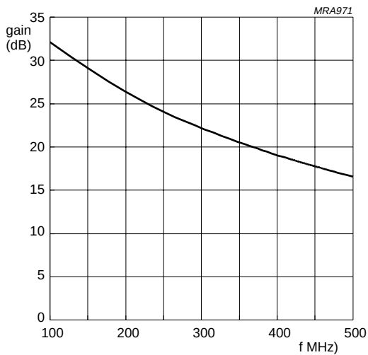
Fig.16 Power gain as a function of frequency, typical values.
