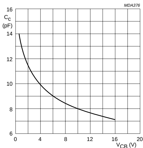
Fig.7 I_E = i_e = 0 ; f = 1 MHz; typ. values.
