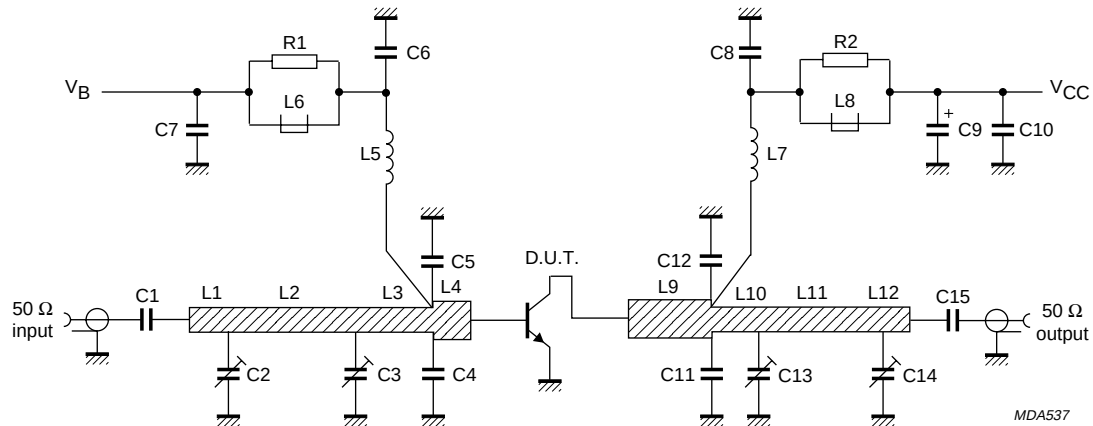
Fig.8 Class-AB test circuit at f = 960 MHz.
