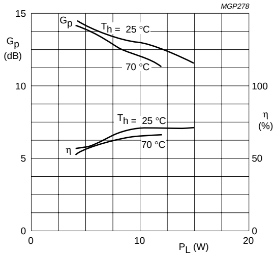
Fig.10 Typical values; V_{CE} = 28\text{ V} ; f = 175\text{ MHz} .
