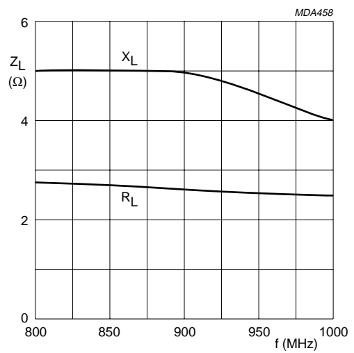
Fig.11 Load impedance; series components; V_{CE} = 24 \text{ V} ; P_L = 15 \text{ W} ; R_{th\ mb-h} = 0.4 \text{ K/W} ; typical values.
