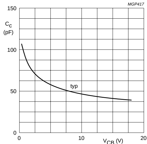
Fig.5 I_E = I_e = 0 ; f = 1\text{ MHz} ; T_j = 25^\circ\text{C} .
