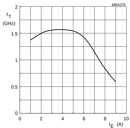
Fig.5 Transition frequency as a function of emitter current, typical values.
