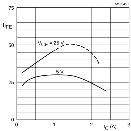
Fig.5 Typical values; T_j = 25^\circ\text{C} .
