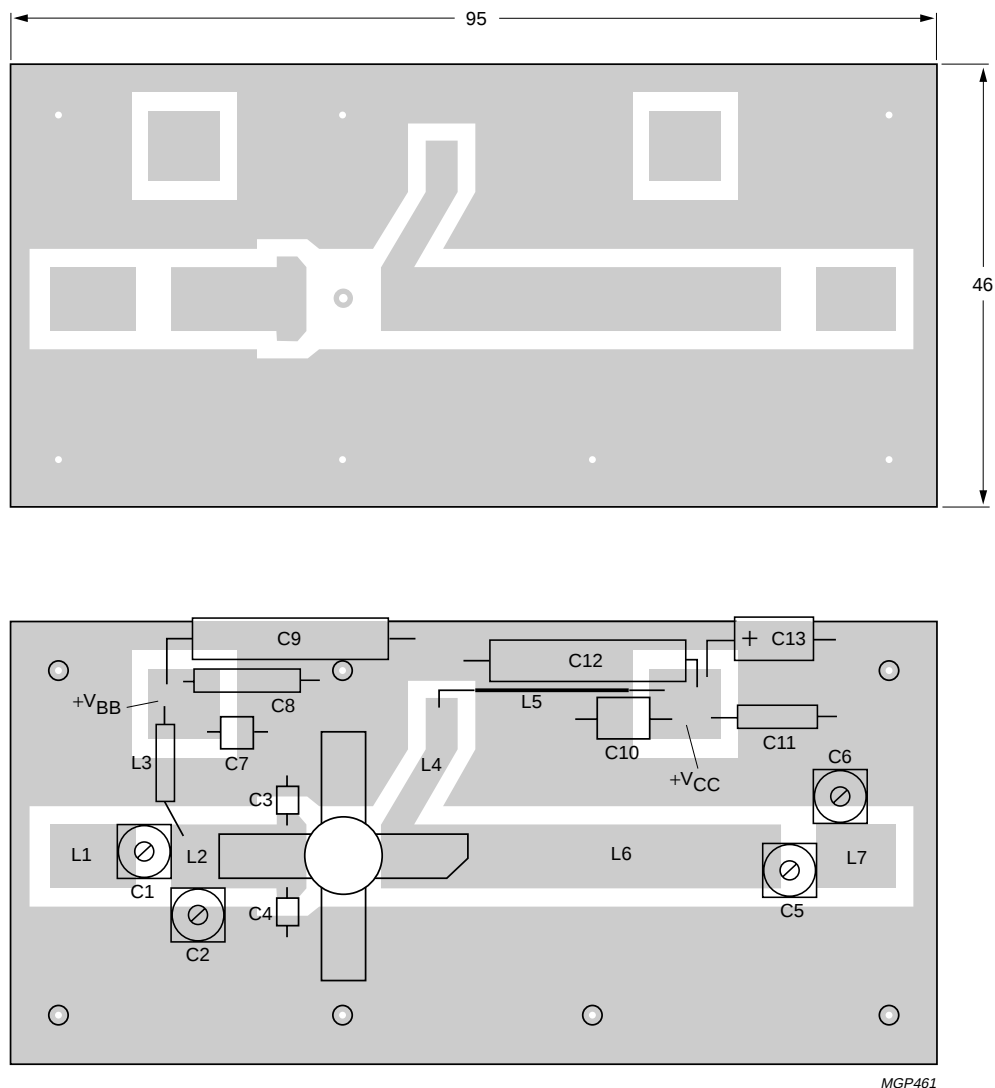
Fig.9 Component layout and printed-circuit board for 860 MHz test circuit.
