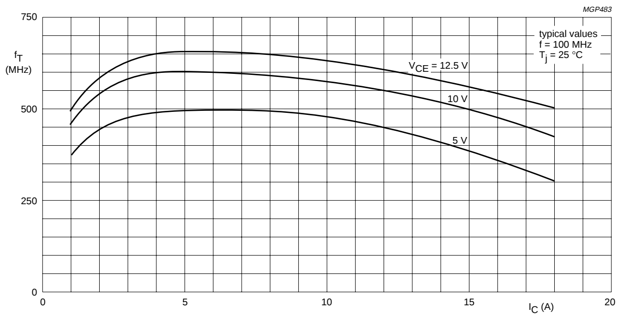
Fig.6 Transition frequency as a function of collector current.
