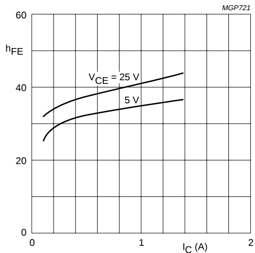
Fig.6 Typical values; T_j = 25\text{ }^{\circ}\text{C} .
