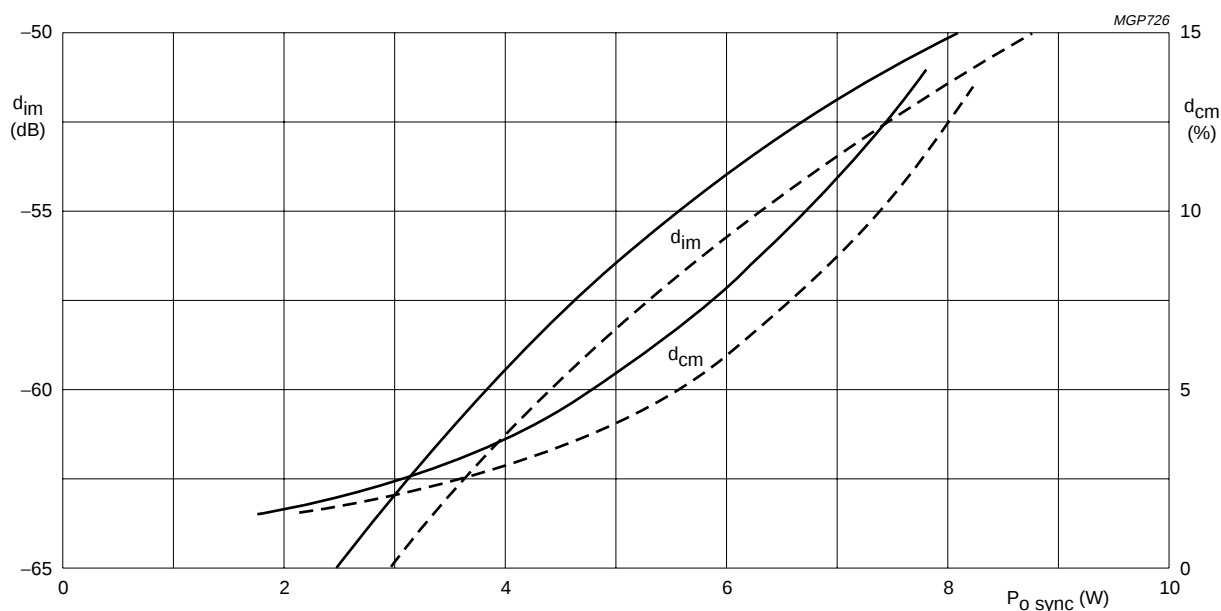
Fig.11 Intermodulation distortion ( d_{im}^{(1)} ) and cross-modulation distortion ( d_{cm}^{(2)} ) as a function of P_{o \text{ sync}} . Typical values; V_{CE} = 25 \text{ V} ; I_C = 850 \text{ mA} ; --- T_h = 25 \text{ }^\circ\text{C} ; — T_h = 70 \text{ }^\circ\text{C} ; f_{\text{vision}} = 860 \text{ MHz} .
