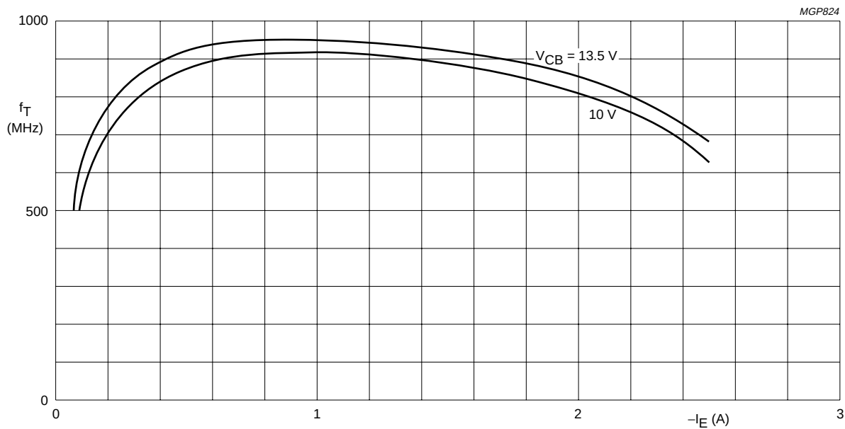
Fig.6 Typical values; f = 100\text{ MHz} ; T_j = 25\text{ }^{\circ}\text{C} .
