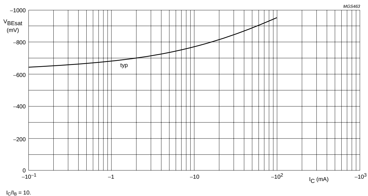
Fig.5 Base-emitter saturation voltage as a function of collector current; typical values.
