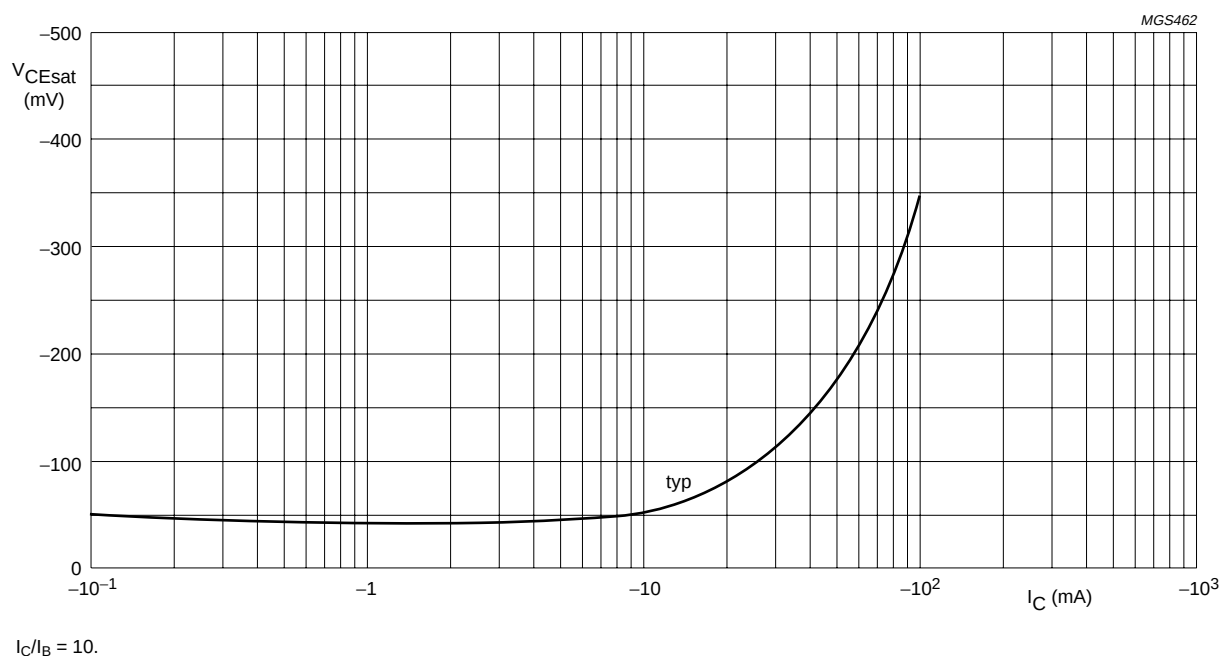
Fig.4 Collector-emitter saturation voltage as a function of collector current; typical values.
