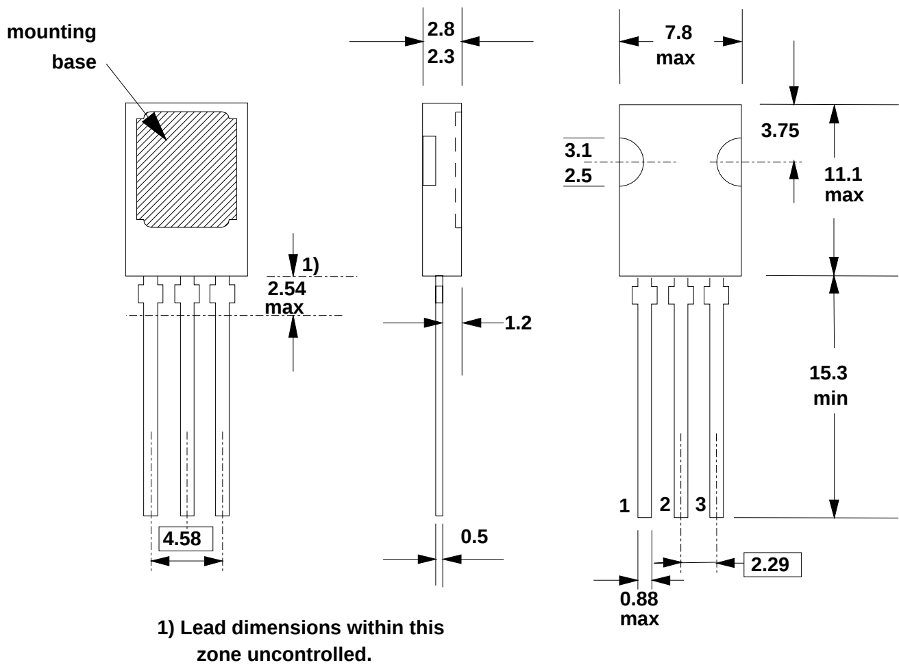
Fig.13. SOT82; pin 2 connected to mounting base.
