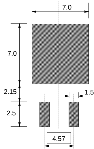
Fig.14. SOT428 : minimum pad sizes for surface mounting.
