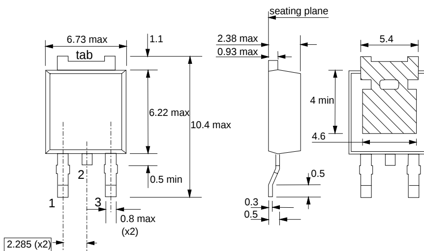
Fig.12. SOT428 : centre pin connected to tab.
