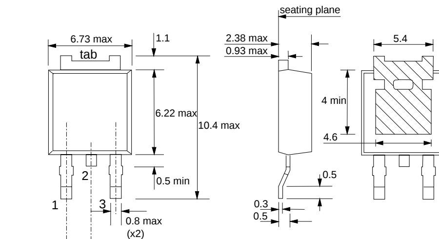
Fig.1. SOT428 : centre pin connected to tab.
