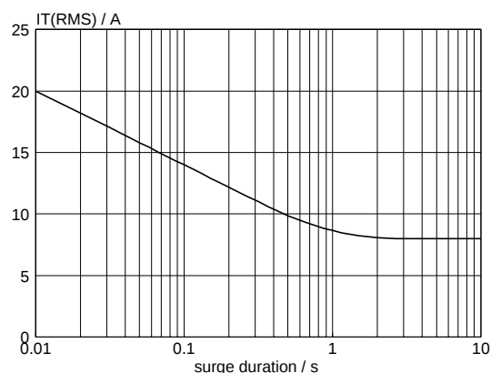
Fig.5. Maximum permissible repetitive rms on-state current I_{T(RMS)} , versus surge duration, for sinusoidal currents, f = 50\text{ Hz} ; T_{hs} \leq 73^\circ\text{C} .
