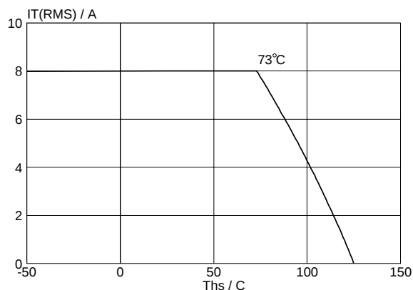
Fig.4. Maximum permissible rms current I_{T(RMS)} , versus heatsink temperature T_{hs} .
