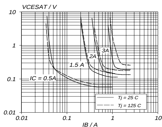
Fig.14. Typical collector-emitter saturation voltage. V_{CESat} = f(I_B) ; parameter I_C
