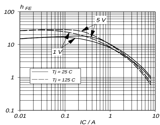
Fig.15. Typical DC current gain. h_{FE} = f(I_C) ; parameter V_{CE}
