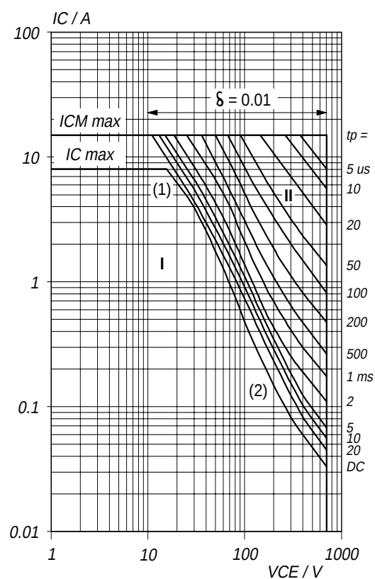
Fig.15. Forward bias safe operating area. T_{mb} = 25^\circ C
