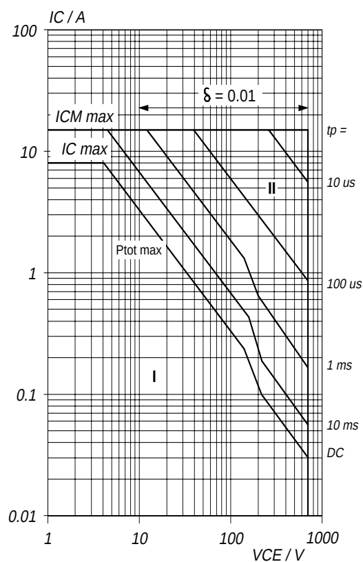
Fig.15. Forward bias safe operating area. T_{hs} = 25^{\circ}\text{C} I Region of permissible DC operation. II Extension for repetitive pulse operation.
