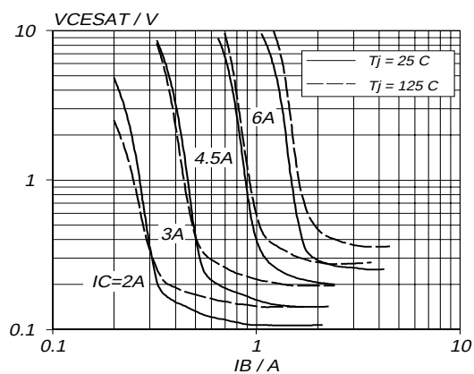
Fig.10. Typical collector-emitter saturation voltage. V_{CE\text{sat}} = f(I_B) ; parameter I_C
