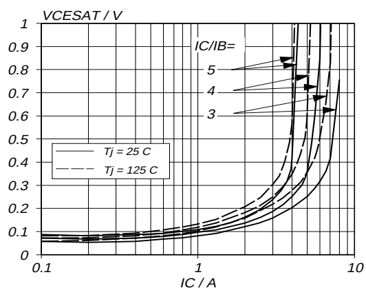
Fig.8. Typical collector-emitter saturation voltage. V_{CE\text{sat}} = f(I_C) ; parameter I_C/I_B
