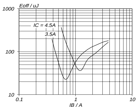
Fig.11. Typical turn-off losses. T_J = 85^\circ\text{C} E_{\text{eff}} = f(I_B) ; parameter I_C ; f = 16\text{ kHz}
