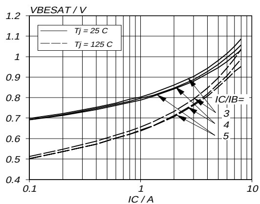
Fig.7. Typical base-emitter saturation voltage. V_{BE\text{sat}} = f(I_C) ; parameter I_C/I_B
