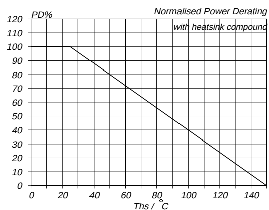
Fig.14. Normalised power dissipation. PD\% = 100 \cdot P_D / P_{D 25^{\circ}\text{C}} = f(T_{hs})
