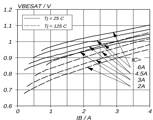
Fig.9. Typical base-emitter saturation voltage. V_{BE\text{sat}} = f(I_B) ; parameter I_C
