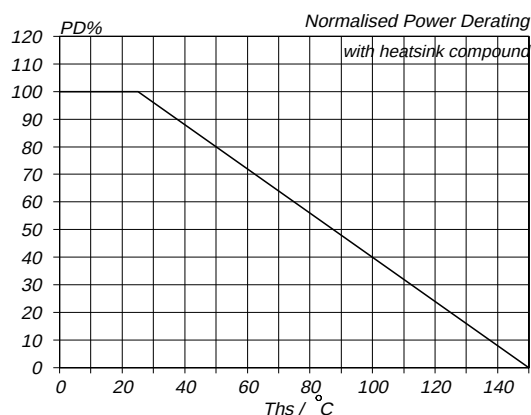
Fig.14. Normalised power dissipation.
