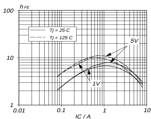
Fig.4. Typical DC current gain. h_{FE} = f(I_C) parameter V_{CE}
