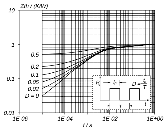
Fig.11. Transient thermal impedance. Z_{\text{th } j\text{-mb}} = f(t) ; parameter D = t_p/T
