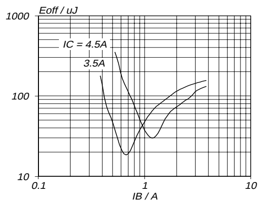
Fig.9. Typical turn-off losses. T_j = 85^\circ\text{C} E_{\text{off}} = f(I_B) ; parameter I_C ; f = 16\text{ kHz}
