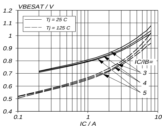
Fig.5. Typical base-emitter saturation voltage. V_{BEsat} = f(I_C) ; parameter I_C/I_B
