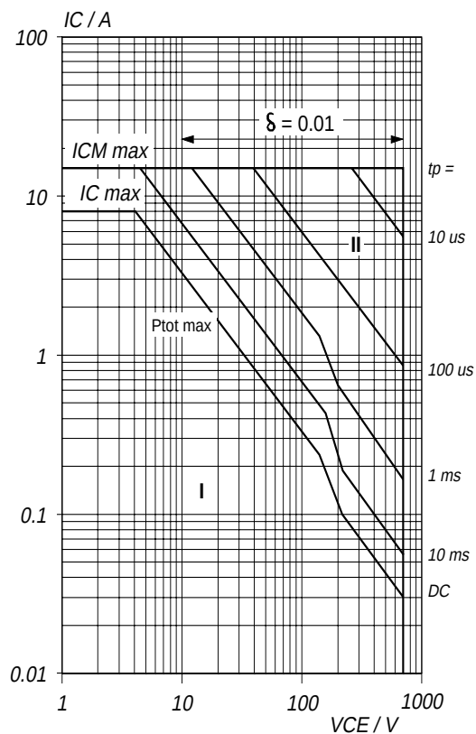
Fig.14. Forward bias safe operating area. T_{hs} = 25^{\circ}\text{C}
