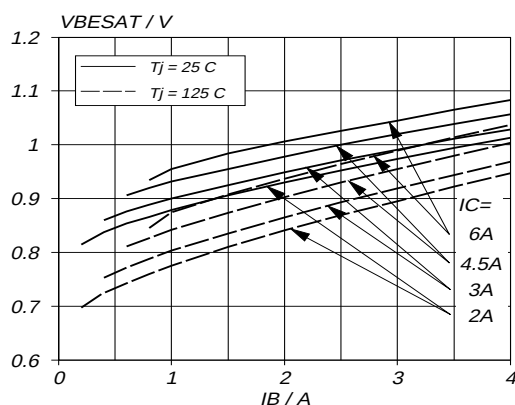
Fig. 7. Typical base-emitter saturation voltage. V_{BE\text{sat}} = f(I_B) ; parameter I_C
