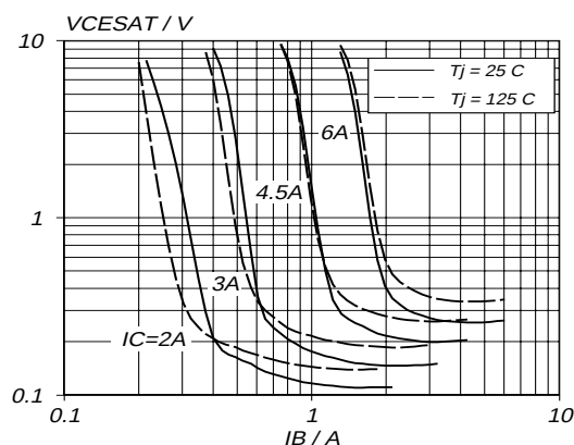
Fig. 8. Typical collector-emitter saturation voltage. V_{CE\text{sat}} = f(I_B) ; parameter I_C
