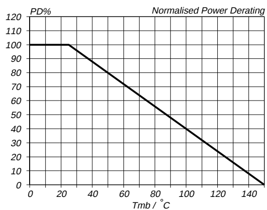
Fig.11. Normalised power dissipation. PD\% = 100 \cdot P_D / P_{D 25^\circ\text{C}} = f(T_{\text{mb}})
