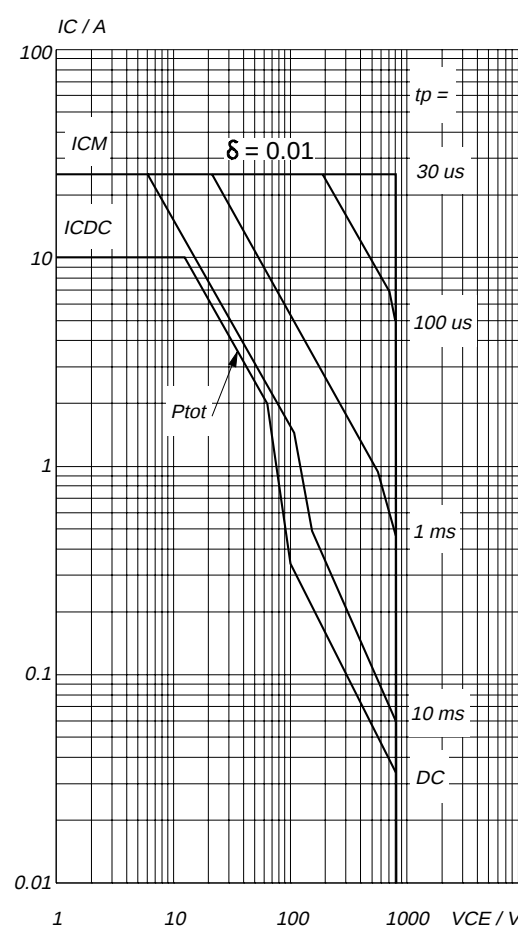
Fig.13. Forward bias safe operating area. T_{\text{mb}} = 25^\circ\text{C} I_{\text{CDC}} \& I_{\text{CM}} = f(V_{\text{CE}}) ; I_{\text{CM}} single pulse; parameter t_p Second-breakdown limits independent of temperature.
