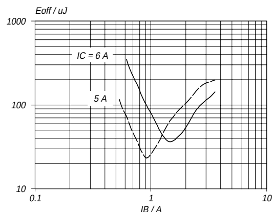
Fig.9. Typical turn-off losses. T_j = 85^\circ\text{C} E_{eff} = f(I_B) ; parameter I_C ; parameter frequency
