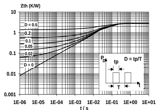
Fig.12. Transient thermal impedance.
