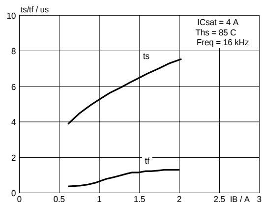
Fig. 12. Typical collector storage and fall time. I_C = 4 \text{ A} ; T_j = 85^\circ\text{C} ; f = 16 \text{ kHz}
