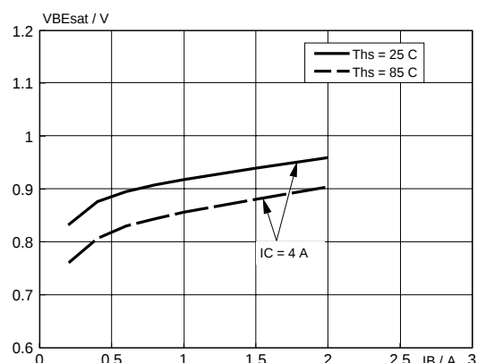
Fig. 11. Typical base-emitter saturation voltage.
