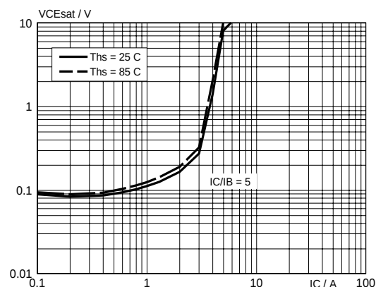
Fig. 10. Typical collector-emitter saturation voltage.
