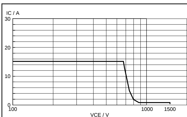
Fig. 9. Reverse bias safe operating area. T_j \leq T_{jmax}
