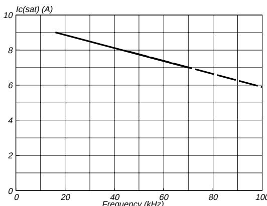
Fig. 12. I_{C\text{sat}} during normal running vs. frequency of operation for optimum performance
