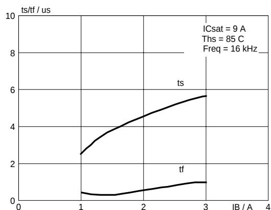
Fig. 9. Typical collector storage and fall time. I_{C\text{sat}} = 9\text{ A}; T_j = 85^\circ\text{C}; f = 16\text{ kHz}
