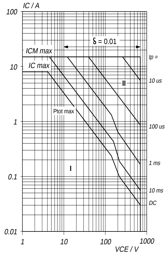
Fig.13. Forward bias safe operating area. T_{hs} = 25^{\circ}\text{C}
