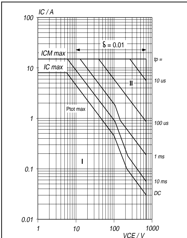
Fig.10. Forward bias safe operating area. T_{hs} = 25^\circ C I Region of permissible DC operation. II Extension for repetitive pulse operation.
