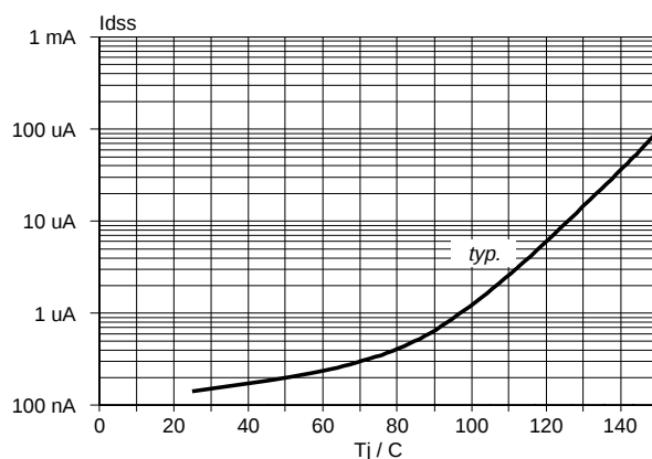
Fig.20. Typical off-state leakage current. I_{DSS} = f(T) ; Conditions: V_{DS} = 40\text{ V} ; I_{IS} = 0\text{ V} .
