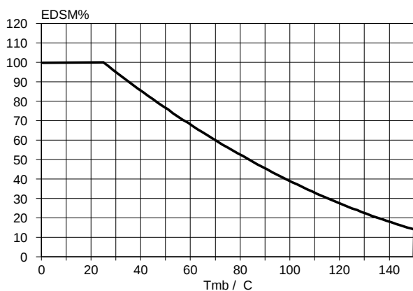
Fig.26. Normalised clamping energy rating. E_{DSM}\% = f(T_{mb}) ; conditions: I_D = 26\text{ A} ; V_{IS} = 5\text{ V}
