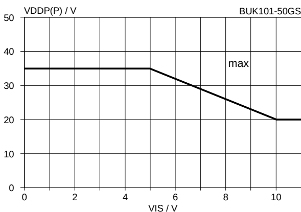
Fig.31. Maximum drain source supply voltage for SC load protection. V_{DDP(P)} = f(V_{IS}) ; T_{mb} \leq 150\text{ }^\circ\text{C}
