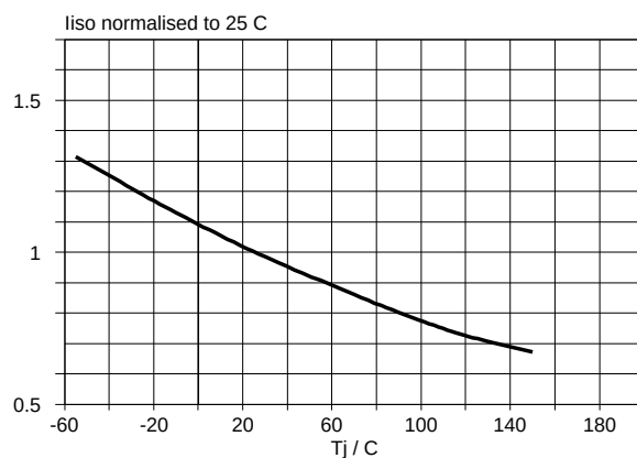
Fig.29. Normalised input current (normal operation). I_{IS}/I_{IS25\text{ }^\circ\text{C}} = f(T_J) ; V_{IS} = 10\text{ V}
