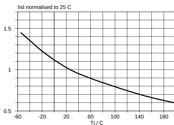
Fig.30. Normalised input current (protection latched). I_{ISL}/I_{ISL25\text{ }^\circ\text{C}} = f(T_J) ; V_{IS} = 10\text{ V}
