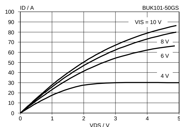
Fig.7. Typical on-state characteristics, T_j = 25^\circ\text{C} . I_D = f(V_{DS}) ; parameter V_{IS} ; t_p = 250\ \mu\text{s}
