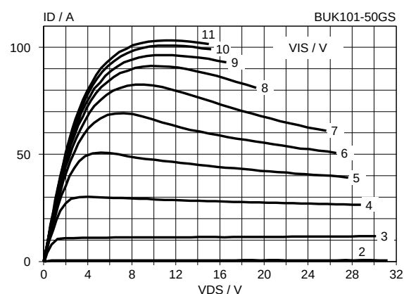
Fig.6. Typical output characteristics, T_j = 25^\circ\text{C} . I_D = f(V_{DS}) ; parameter V_{IS} ; t_p = 250\ \mu\text{s} & t_p < t_{dsc}
