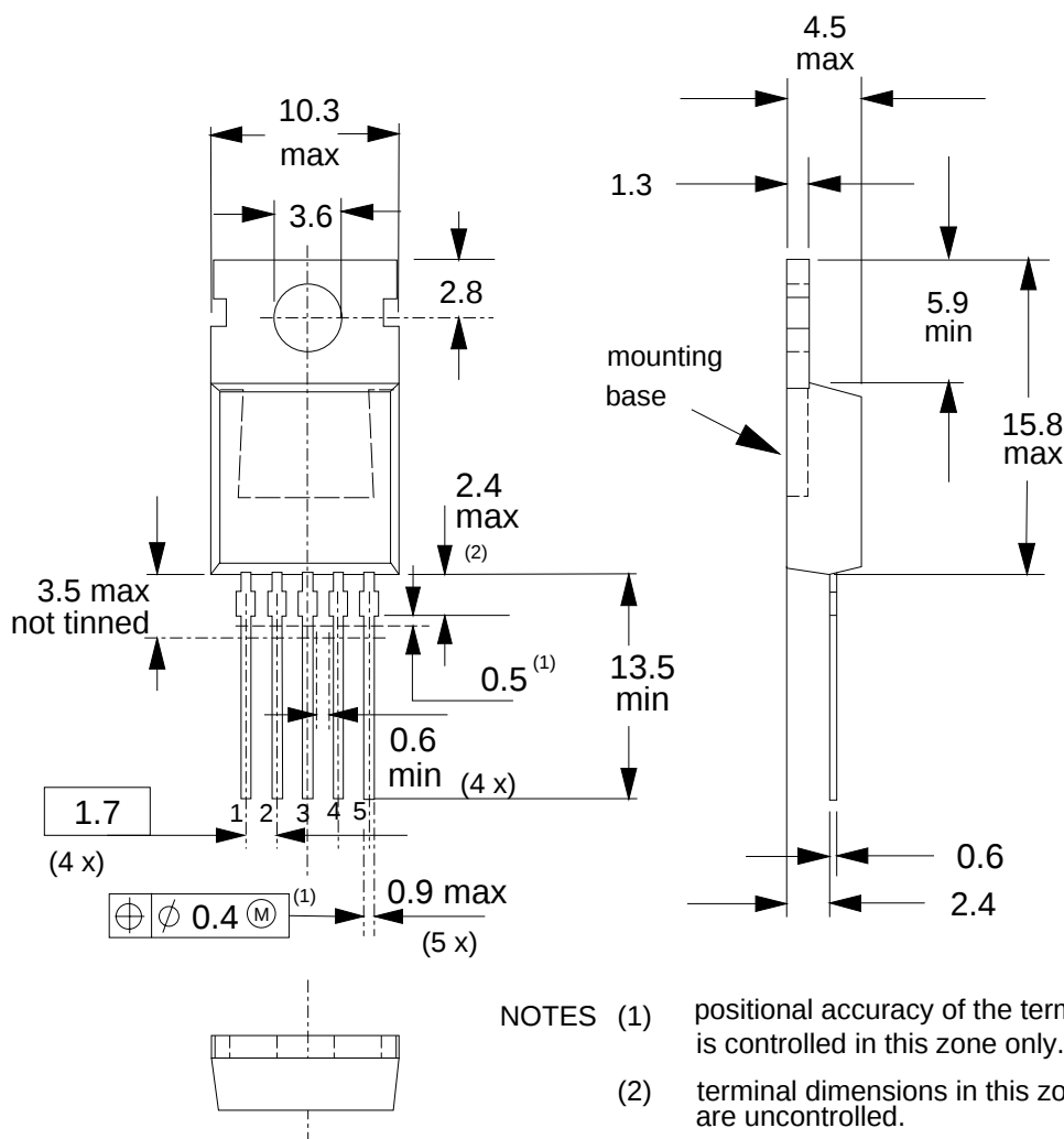
Fig.33. SOT263 ( 5-pin TO220 );
