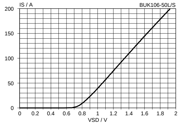
Fig. 25. Typical reverse diode current, T_J = 25^\circ \text{C} . I_S = f(V_{SDS}) ; conditions: V_{IS} = 0 \text{ V} ; t_p = 250 \mu\text{s}
