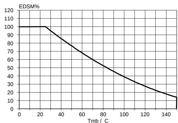
Fig. 26. Normalised limiting clamping energy. E_{DSM}\% = f(T_{mb}) ; conditions: I_D = 27 \text{ A}
