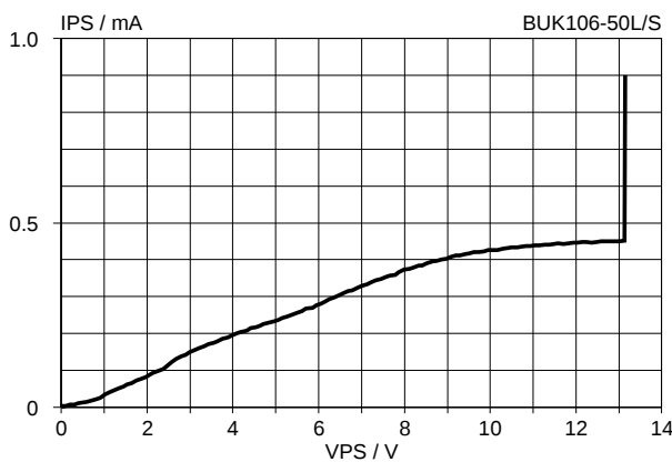
Fig. 23. Typical DC protection supply characteristics. I_{PS} = f(V_{PS}) ; normal or overload operation; T_J = 25^\circ \text{C}
