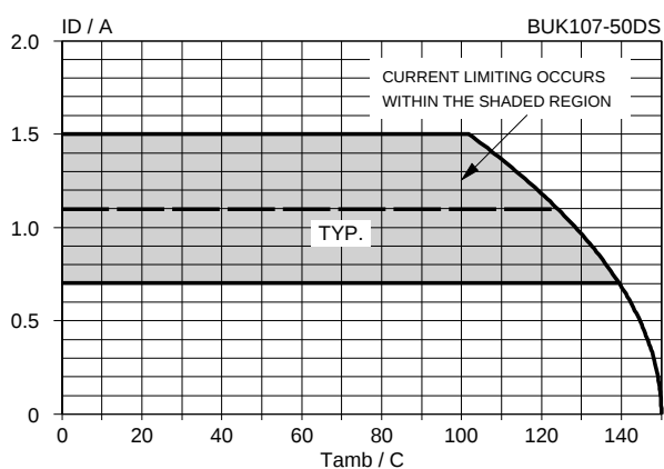
Fig.3. Continuous drain current. I_D = f(T_{amb}); \text{condition: } I_f = 1.5\text{ mA}
