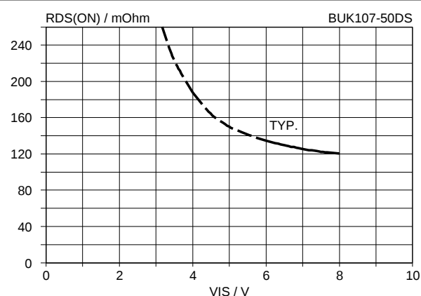
Fig.6. Typical on-state resistance, T_j = 25^\circ\text{C} . R_{DS(ON)} = f(V_{DS}); \text{conditions: } I_D = 100\text{ mA}, t_p = 300\text{ }\mu\text{s}
