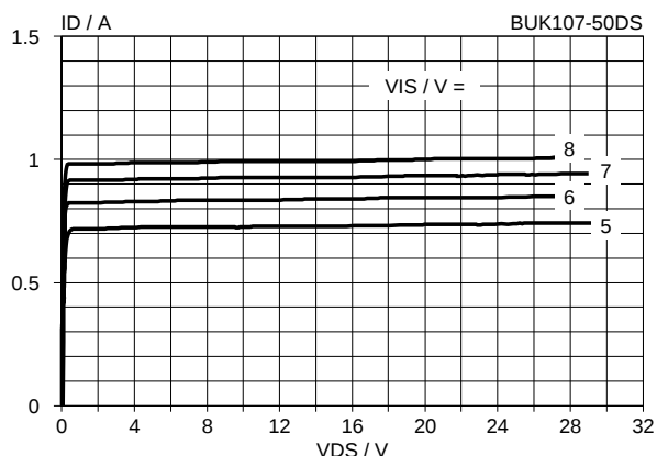
Fig.4. Typical on-state characteristics, T_j = 25^\circ\text{C} . I_D = f(V_{DS}); \text{parameter } V_{GS}; t_p = 300\text{ }\mu\text{s}
