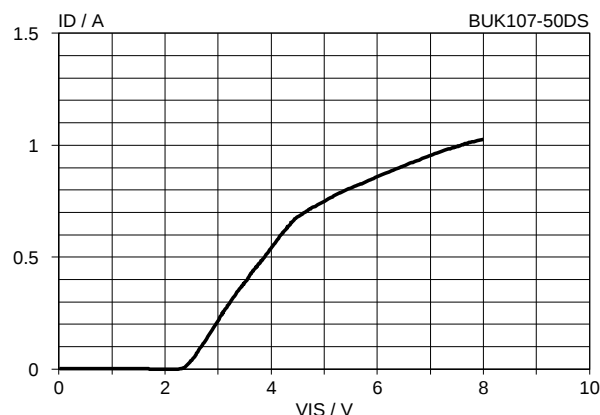
Fig.7. Typical transfer characteristics, T_j = 25^\circ\text{C} . I_D = f(V_{GS}); \text{conditions: } V_{DS} = 10\text{ V}, t_p = 300\text{ }\mu\text{s}
