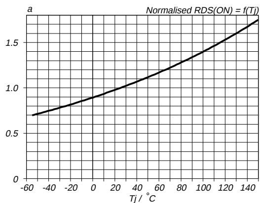
Fig.5. Normalised drain-source on-state resistance. a = R_{DS(ON)} / R_{DS(ON)}(25^\circ\text{C}) = f(T_j); I_D = 100\text{ mA}; I_f = 1.5\text{ mA}
