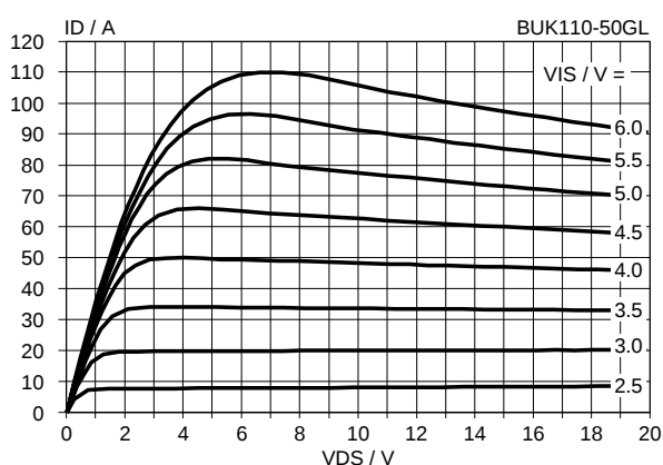
Fig.6. Typical output characteristics, T_j = 25^\circ\text{C} . I_D = f(V_{DS}) ; parameter V_{IS} ; t_p = 250\ \mu\text{s} & t_p < t_{dsc}
