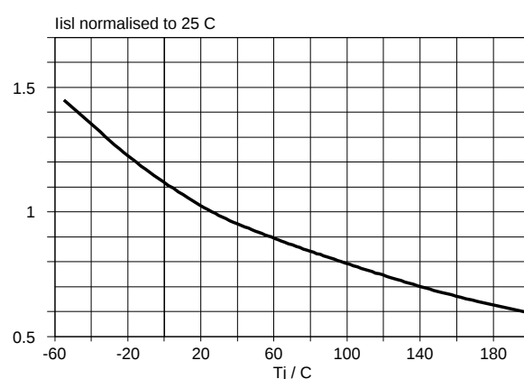
Fig.30. Normalised input current (protection latched). I_{ISL}/I_{ISL25^\circ\text{C}} = f(T_J) ; V_{IS} = 5\text{ V}
