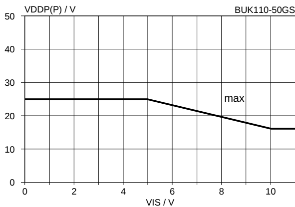
Fig.31. Maximum drain source supply voltage for SC load protection. V_{DDP(P)} = f(V_{IS}) ; T_{mb} \leq 150^\circ\text{C}
