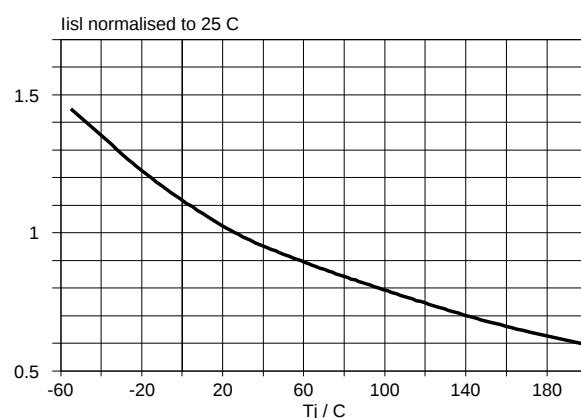
Fig.30. Normalised input current (protection latched). I_{ISL}/I_{ISL25^\circ\text{C}} = f(T_J) ; V_{IS} = 10\text{ V}
