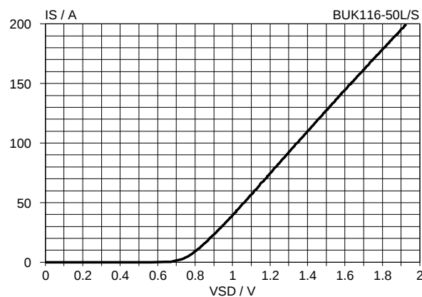
Fig.25. Typical reverse diode current, T_J = 25^\circ \text{C} . I_S = f(V_{DS}) ; conditions: V_{IS} = 0 \text{ V} ; t_p = 250 \mu\text{s}
