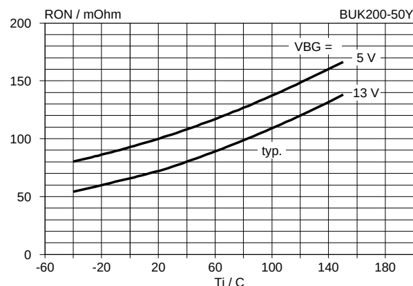
Fig. 9. Typical on-state resistance, t_p = 300\ \mu\text{s} . R_{ON} = f(T_j) ; parameter V_{BG} ; condition I_L = 1\ \text{A}
