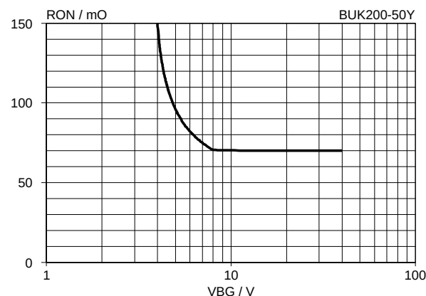
Fig. 8. Typical on-state resistance, T_j = 25^\circ\text{C} . R_{ON} = f(V_{BG}) ; conditions: I_L = 5\ \text{A} ; t_p = 300\ \mu\text{s}
