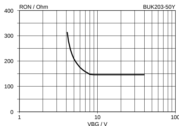
Fig.8. Typical on-state resistance, T_j = 25^\circ\text{C} . R_{ON} = f(V_{BG}) ; conditions: I_L = 2\ \text{A} ; t_p = 300\ \mu\text{s}
