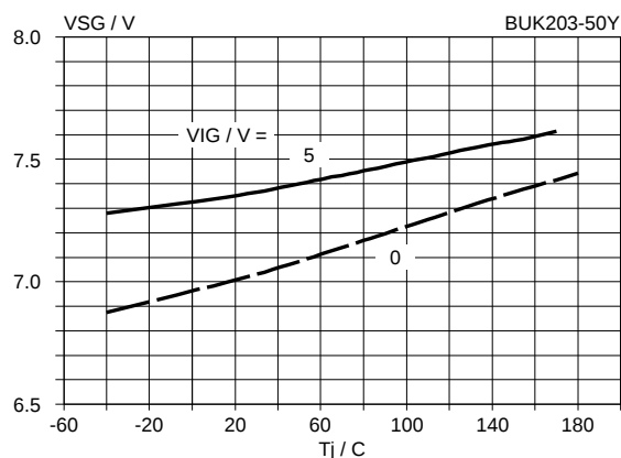
Fig.22. Typical status clamping voltage, V_{SG} = f(T_j) . parameter V_{IG} ; conditions I_S = 100 \mu A , V_{BG} = 13 V
