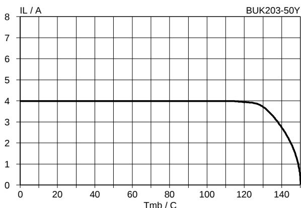
Fig.6. Limiting continuous on-state load current. I_L = f(T_{mb}) ; conditions: V_{IG} = 5\ \text{V} , V_{BG} = 13\ \text{V}
