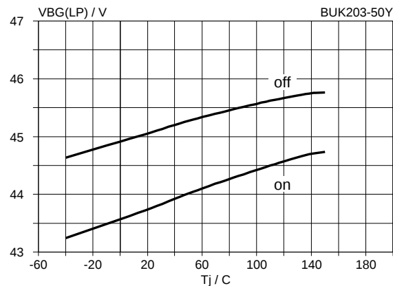
Fig.25. Supply typical overvoltage thresholds. V_{BG(LP)} = f(T_j) ; conditions V_{IG} = 5 V ; I_L = 100 mA
