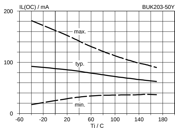
Fig.23. Low load current detection threshold. I_{L(OC)} = f(T_j) ; conditions V_{IG} = 5 V ; V_{BG} = 13 V
