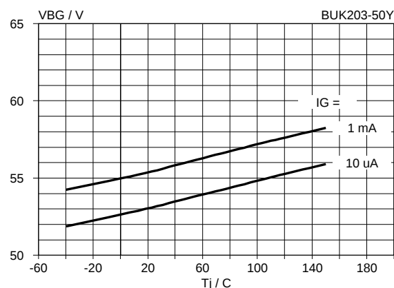
Fig.26. Typical battery to ground clamping voltage. V_{BG} = f(T_j) ; parameter I_G
