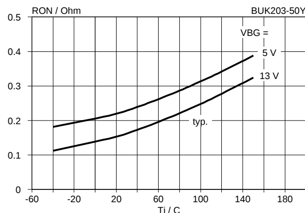
Fig.9. Typical on-state resistance, t_p = 300\ \mu\text{s} . R_{ON} = f(T_j) ; parameter V_{BG} ; condition I_L = 0.5\ \text{A}
