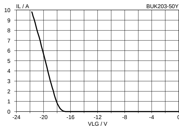
Fig.27. Typical negative load clamping characteristic. I_L = f(V_{LG}) ; conditions V_{IG} = 0 V , t_p = 300 \mu s , 25 ^\circ C
