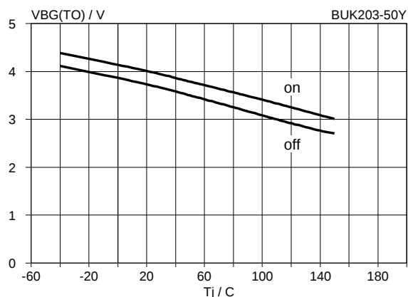
Fig.24. Supply typical undervoltage thresholds. V_{BG(TO)} = f(T_j) ; conditions V_{IG} = 3 V ; I_L = 100 mA
