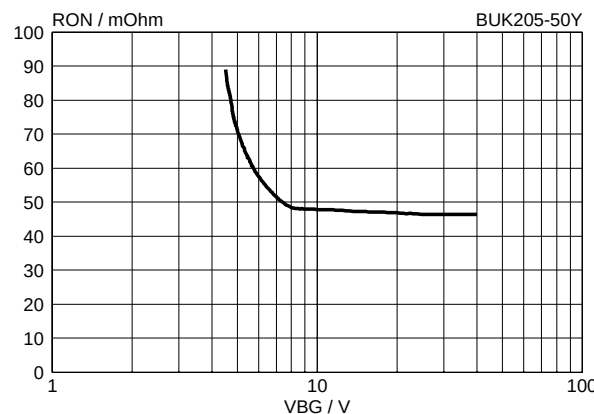
Fig.8. Typical on-state resistance, T_j = 25^\circ\text{C} . R_{ON} = f(V_{BG}) ; conditions: I_L = 7.5\ \text{A} ; t_p = 300\ \mu\text{s}
