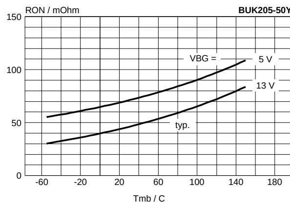
Fig.9. Typical on-state resistance, t_p = 300\ \mu\text{s} . R_{ON} = f(T_j) ; parameter V_{BG} ; condition I_L = 1.5\ \text{A}
