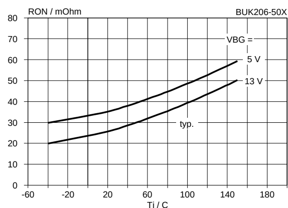
Fig.9. Typical on-state resistance, t_p = 300\ \mu\text{s} . R_{ON} = f(T_j) ; parameter V_{BG} ; condition I_L = 2\ \text{A}
