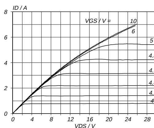
Fig.5. Typical output characteristics, T_j = 25\ ^\circ C . I_D = f(V_{DS}) ; parameter V_{GS}
