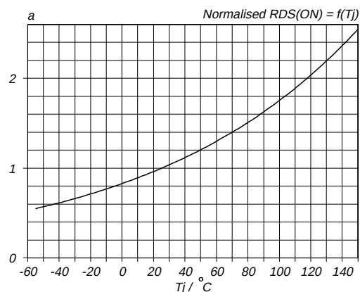
Fig.9. Normalised drain-source on-state resistance. a = R_{DS(ON)} / R_{DS(ON)25^\circ\text{C}} = f(T_j) ; I_D = 1.0 \text{ A} ; V_{GS} = 10 \text{ V}
