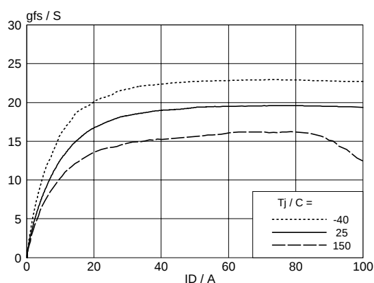
Fig. 8. Typical transconductance, T_j = 25 \text{ °C} . g_{fs} = f(I_D) ; conditions: V_{DS} = 10 \text{ V}
