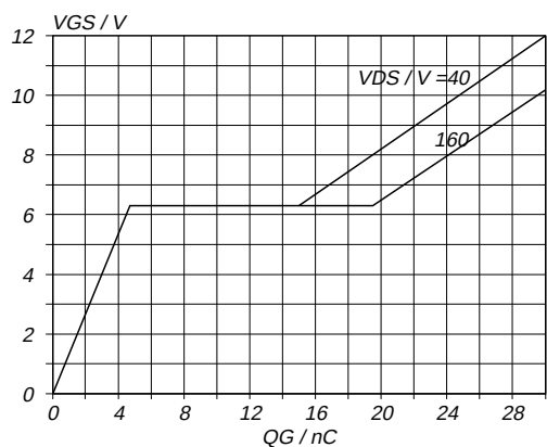
Fig.13. Typical turn-on gate-charge characteristics. V_{GS} = f(Q_G) ; conditions: I_D = 9.2 A; parameter V_{DS}
