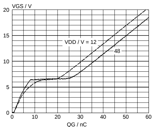
Fig.13. Typical turn-on gate-charge characteristics. V_{GS} = f(Q_G) ; conditions: I_D = 43 A; parameter V_{DS}
