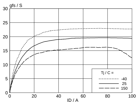
Fig.8. Typical transconductance, T_J = 25 °C. g_{fs} = f(I_D) ; conditions: V_{DS} = 10 V
