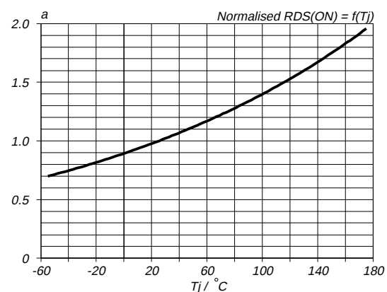
Fig.9. Normalised drain-source on-state resistance. a = R_{DS(ON)} / R_{DS(ON)25\text{ °C}} = f(T_J) ; I_D = 20 A; V_{GS} = 5 V
